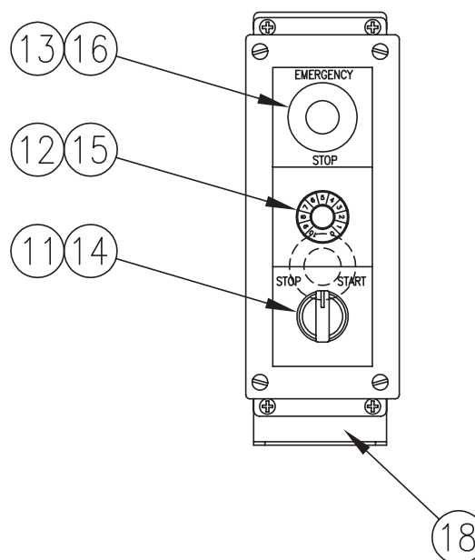
VERTICAL MOUNT
