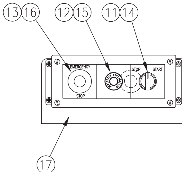
HORIZONTAL MOUNT
